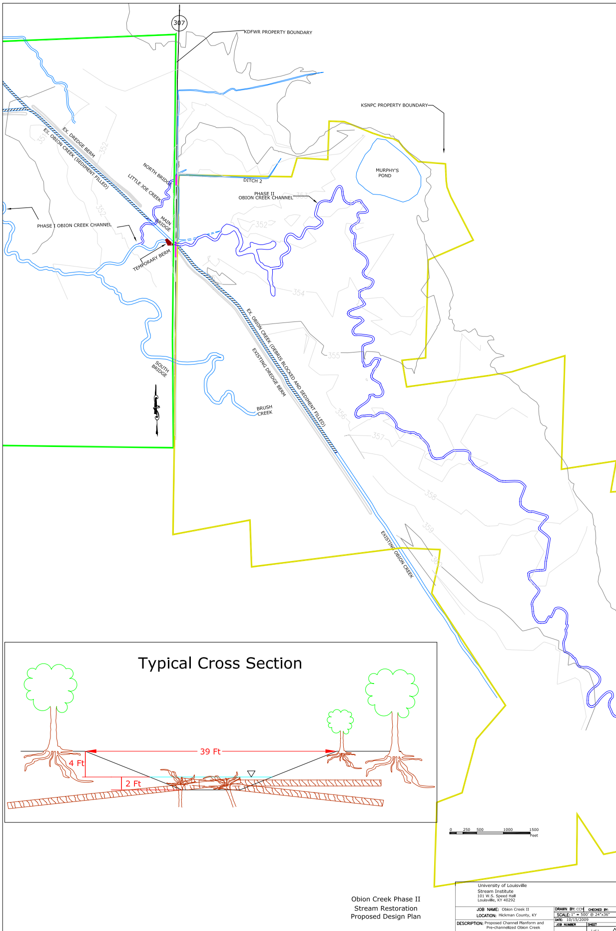
Figure 24 Obion and Little Joe restoration plan showing the temporary berm (in magenta) and a typical cross section at the location of a grade control structure.
